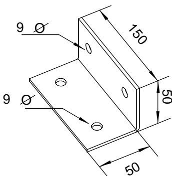
TYPE D MULTI PURPOSE BRACKET 50 X 50 X 1 00 X 2.5mm
