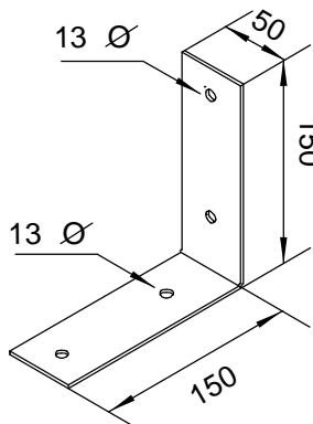
TYPE E MULTI-PURPOSE BRACKET 150 X 150 X 2.5m
