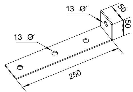
TYPE H MULTI PURPOSE BRACKET 50 X 250 X 3.0mm
