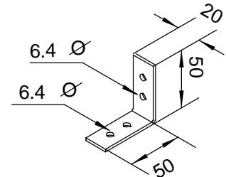
TYPE C MULTI-PURPOSE BRACKET 50 X 50 X 20 X 2.5 mm
