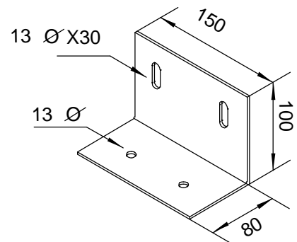
TYPE F MULTI-PURPOSE BRACKET 150 X 80 X 100 X 2.5mm
