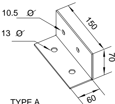
TYPE A MULTI PURPOSE BRACKET 60 X 70 X 150 LG X 2.5 mm
