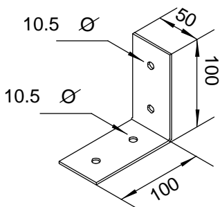
TYPE G MULTI-PURPOSE BRACKET 100 X 100 X 2.5mm
