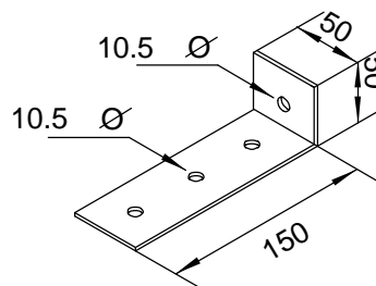
TYPE J MULTI PURPOSE BRACKET 50 X 150 X 2.5mm
