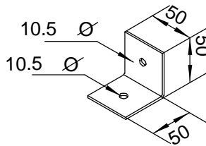
TYPE B MULTI PURPOSE BRACKET 50 X 50 X 50 X 2.5mm
